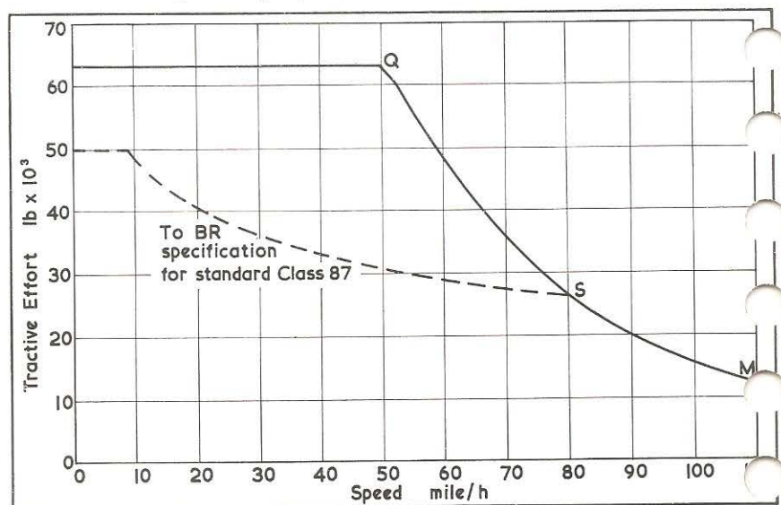
Fig. 3. Tractive effort/speed characteristics of Class 87 No. 87101 showing the latter's performance which is well above that of the standard Class 87 until the point 'S' is reached
