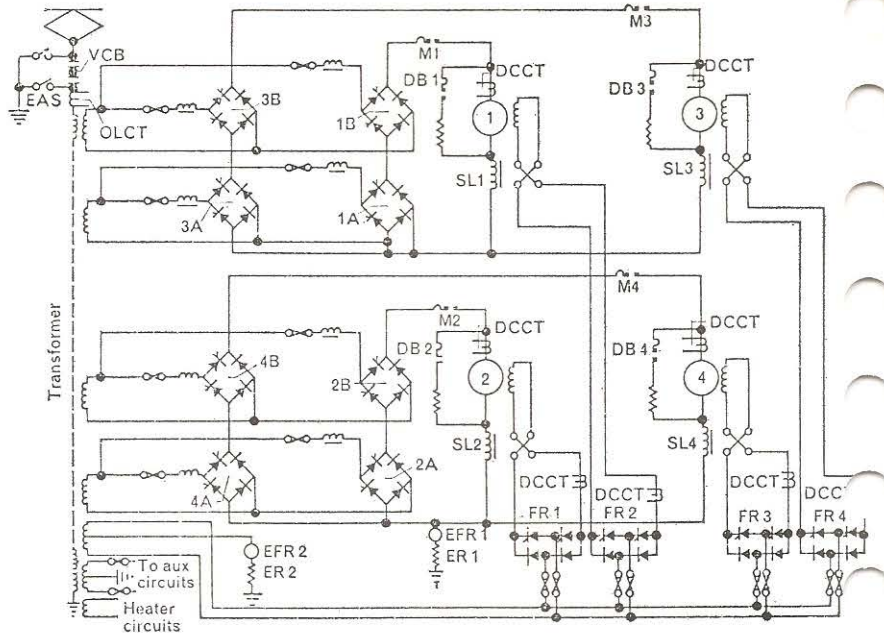
Fig. 2. Schematic circuit diagram of Class 87 No. 87 locomotive
